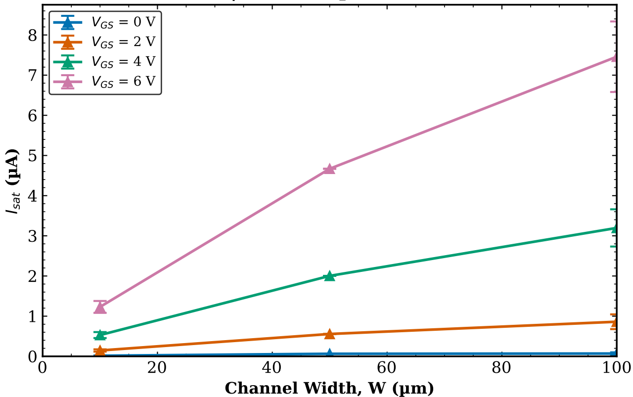
TFT1 Combined (Tr. 1 & 2) I_{sat} vs W | L = 160\text{ }\mu\text{m} (mean \pm std)
